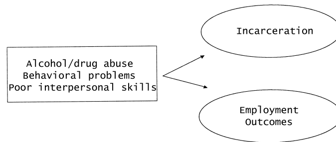
FIG. 2.—Model of spurious effects
